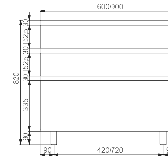
CABINET - 1 DEEP DRAWERS + 2 STD DRAWERS E071000127 (Code 60 cm) E071000109 (Code 90 cm)
