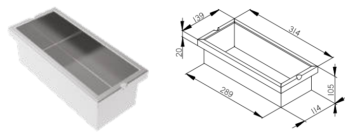
CONTENITORE CN314-105 Container CN314-105
