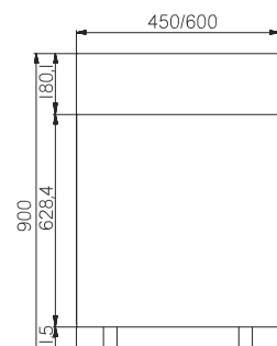
CABINET - 1 DOOR E071000119 (Code 45 cm) E071000124 (Code 60 cm)
