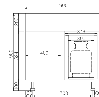
CABINET - 2 DOORS WITH COMPARTMENT FOR GAS CYLINDER E071000120 (Code 90 cm)
