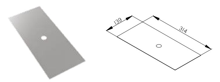
COPERCHIO VASCHETTA CPCN314 Vegetable basin cover CPCN314
