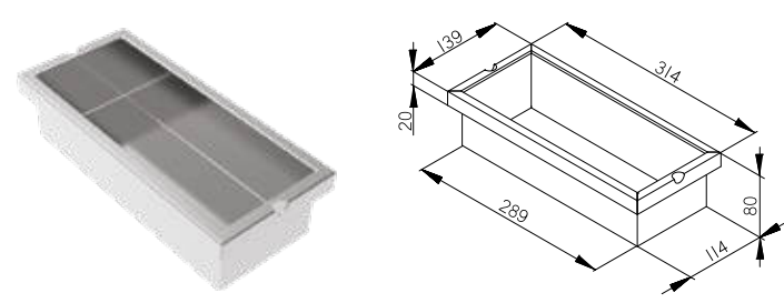
CONTENITORE CN314-80 Container CN314-80
