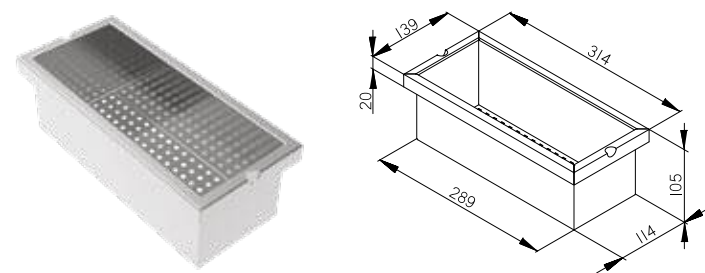
CONTENITORE CN314-105F Container CN314-105F
