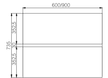
WALL CABINET - 2 VASISTAS E071000134 (Code 60 cm) E071000113 (Code 90 cm)
