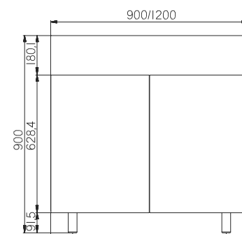
CABINET - 2 DOORS E071000117 (Code 90 cm) E071000123 (Code 120 cm)
