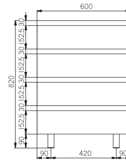
CABINET - 4 DRAWERS E071000107 (Code 60 cm)
