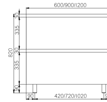
CABINET - 2 DEEP DRAWERS E071000128 (Code 60 cm) E071000110 (Code 90 cm) E071000129 (Code 120 cm)
