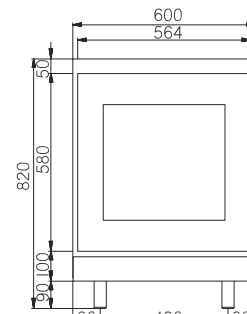
OVEN CABINET E071000106 (Code 60 cm)
