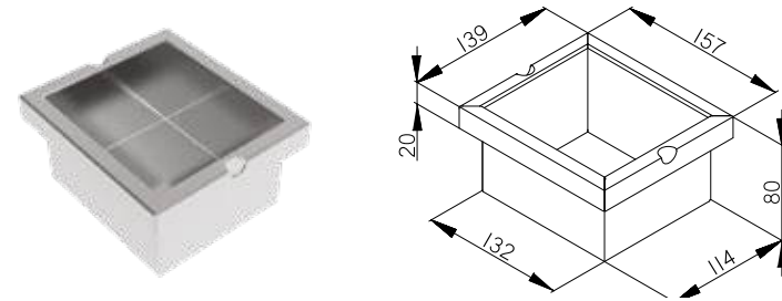
CONTENITORE PICCOLO CN157 Small container CN157
