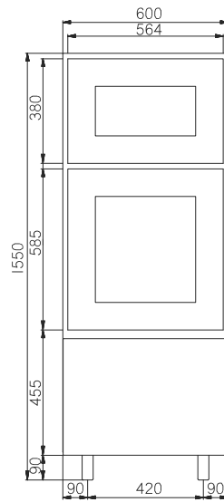
COLUMN SYSTEM E071000108 (Code 60 cm)
