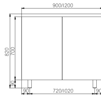
CABINET - 2 DOOR E071000125 (Code 60 cm) E071000103 (Code 90 cm) E071000126 (Code 120 cm)
