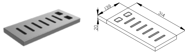
SUPPORTO COLTELLI SPCL Knife rack SPCL
