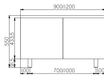
CABINET - 2 DOORS - BBQ E071000118 (Code 90 cm) E071000122 (Code 120 cm)
