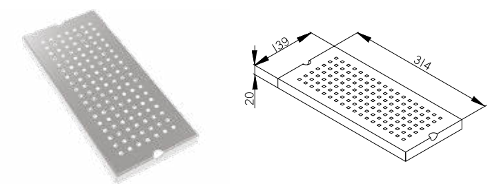
SUPPORTO BICCHIERI SCBC Glass rack SCBC
