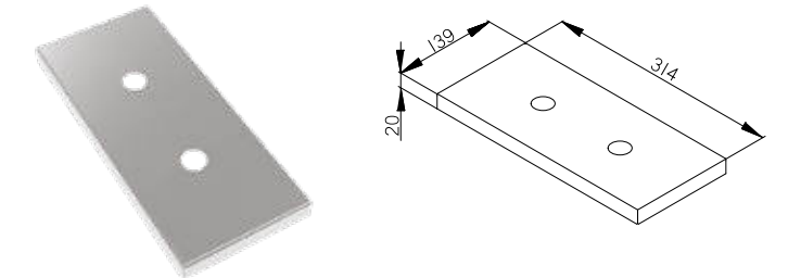
SUPPORTO BICCHIERI SCBC Glass rack SCBC
